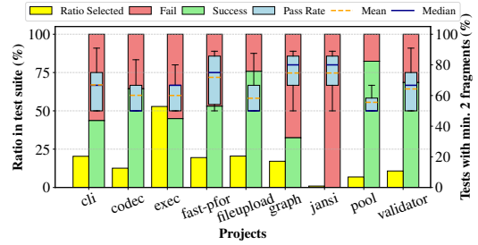
Fig. 6. Effectiveness of test decomposition in ALPHA-TRANS for validating earlier fragments in failing tests. decomposed test fragments were useful in helping
